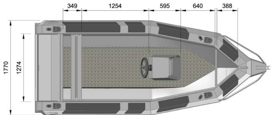
Boat shown with optional extras
